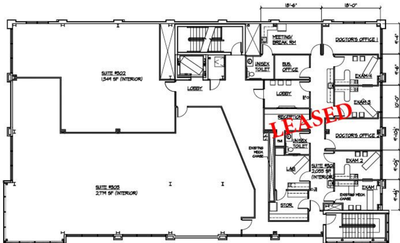
THIRD FLOOR TENANT SCHEMATIC SCALE: 1/4"=1'-0"
